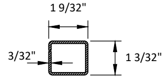
⑫ REINFORCEMENT
