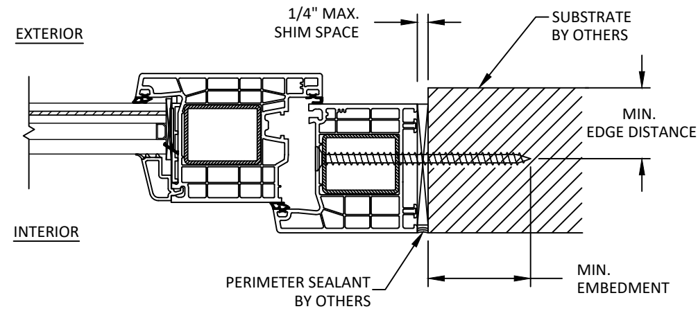
A 7 ANCHOR DETAIL THROUGH FRAME (JAMB)
